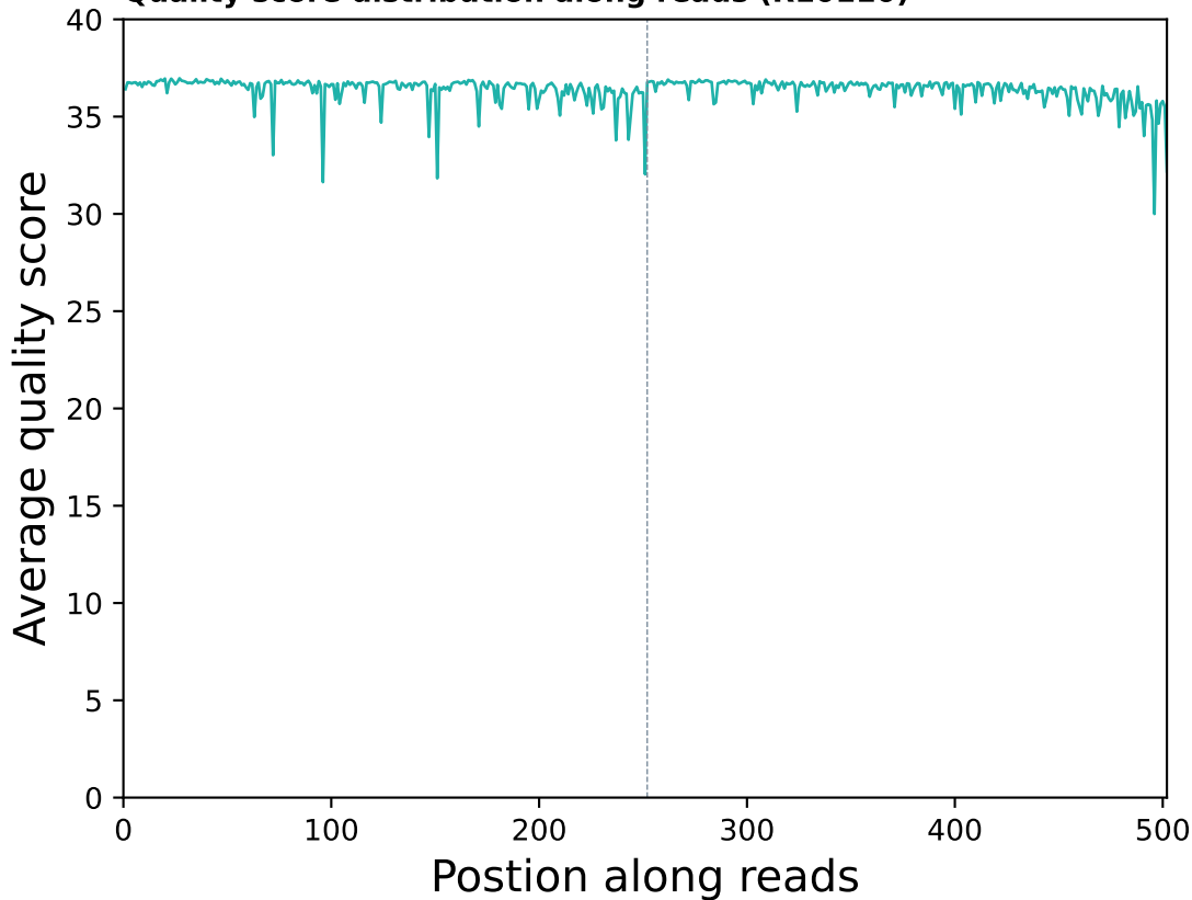
Quality score distribution along reads (R10110)
